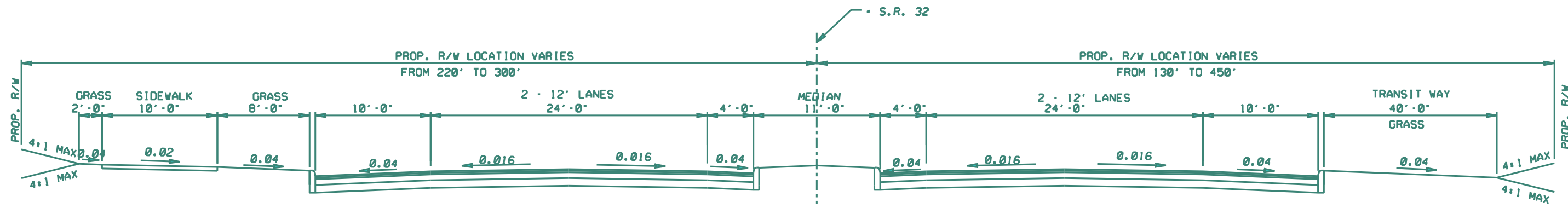
CONCEPTUAL TYPICAL SECTION - SEGMENT 2 & 3 PROFILE @5.00% MAX U.S. 50 TO ANCOR CONNECTOR
