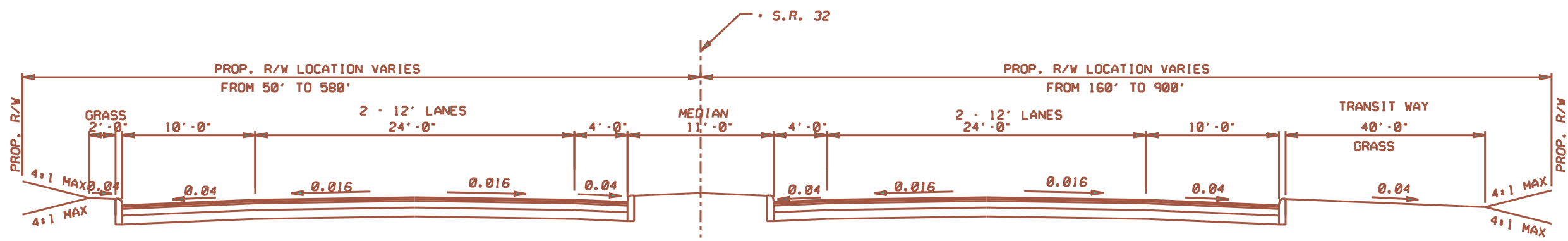
CONCEPTUAL TYPICAL SECTION - SEGMENT 3 PROFILE @5.00% MAX ANCOR CONNECTOR TO MT. CARMEL - TOBASCO ROAD
