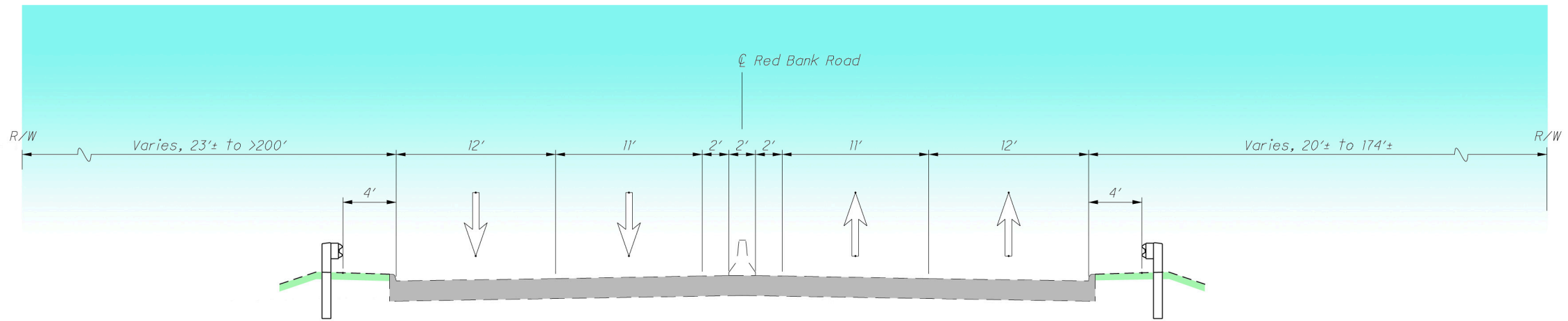
RED BANK EXPRESSWAY TYPICAL SECTION Between Duck Creek Road & Interstate 71
