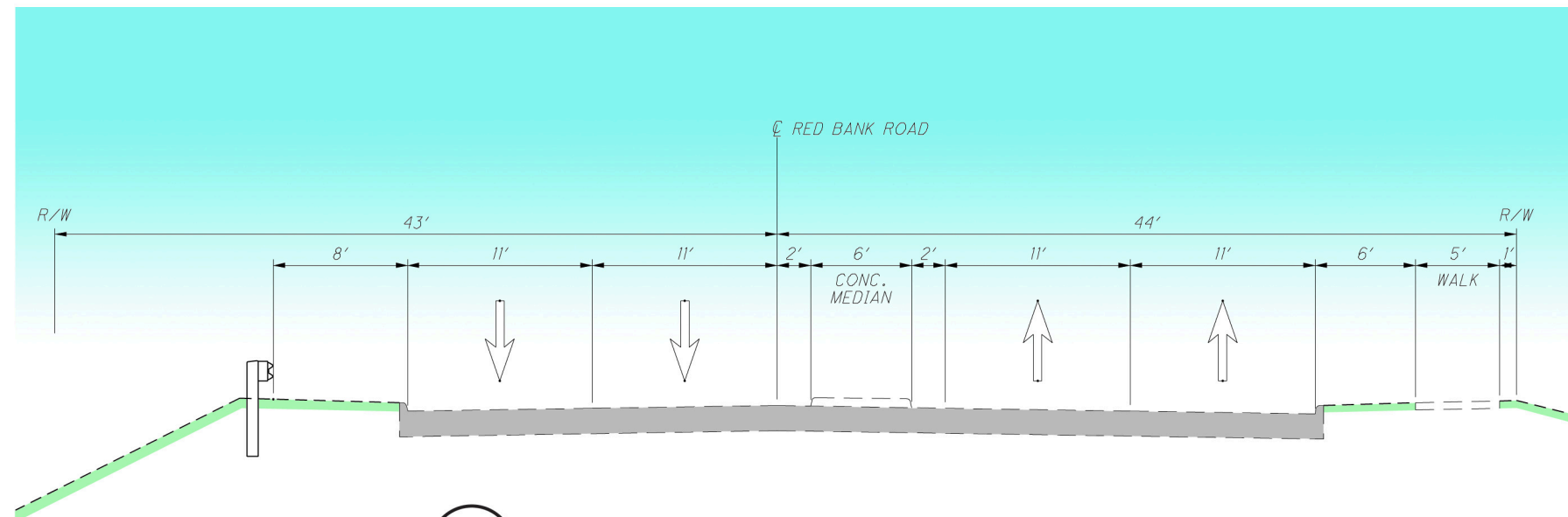
B RED BANK ROAD TYPICAL SECTION Erie Avenue to Indiana & Ohio Railroad (Near Gorilla Glue)
